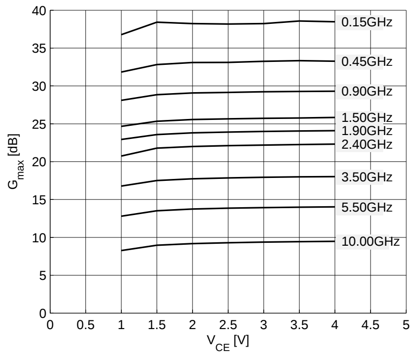
Figure 5-14 Maximum Power Gain G_{\max} = f(V_{CE}) , I_C = 25\text{ mA} , f = \text{Parameter in GHz}
