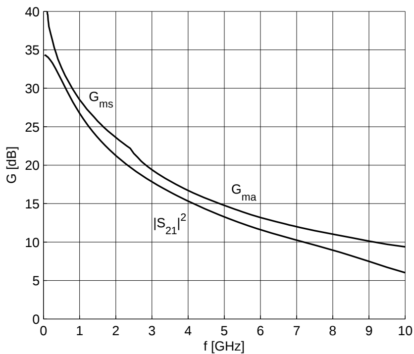
Figure 5-12 Gain G_{ma} , G_{ms} , |S_{21}|^2 = f(f) , V_{CE} = 3 V, I_C = 25 mA
