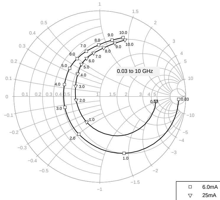
Figure 5-15 Input Matching S_{11} = f(f) , V_{CE} = 3\text{ V} , I_C = 6 / 25\text{ mA}
